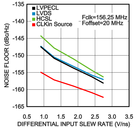
Noise Floor vs. CLKin Slew Rate @ 156.25 MHz
