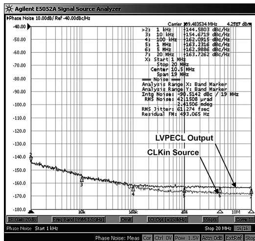
LVPECL Phase Noise @ 100 MHz (Note 26)
