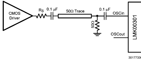
FIGURE 5. Driving OSCin with a Single-Ended Input
