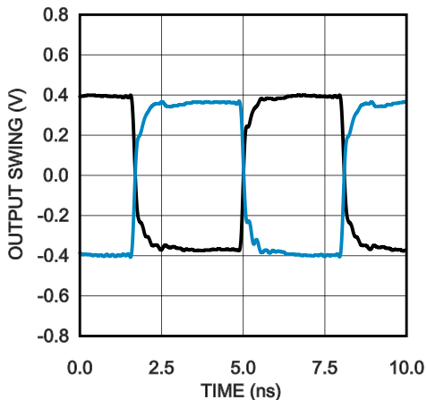
LVPECL Output Swing @ 156.25 MHz
