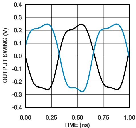
LVPECL Output Swing @ 1.5 GHz
