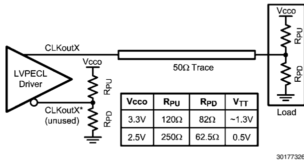
FIGURE 14. Single-Ended LVPECL Operation, DC Coupling, Thevenin Equivalent
