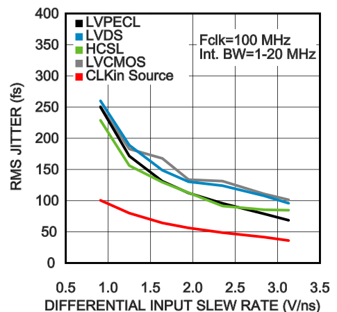
RMS Jitter vs. CLKin Slew Rate @ 100 MHz (Note 26)
