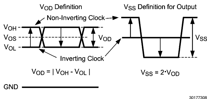
FIGURE 2. Two Different Definitions for Differential Output Signals
