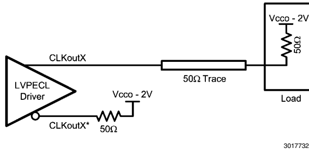
FIGURE 13. Single-Ended LVPECL Operation, DC Coupling
