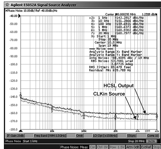
HCSL Phase Noise @ 100 MHz (Note 26)
