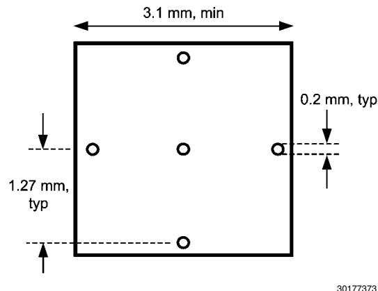
FIGURE 17. Recommended Land and Via Pattern
