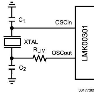
FIGURE 6. Crystal Interface
