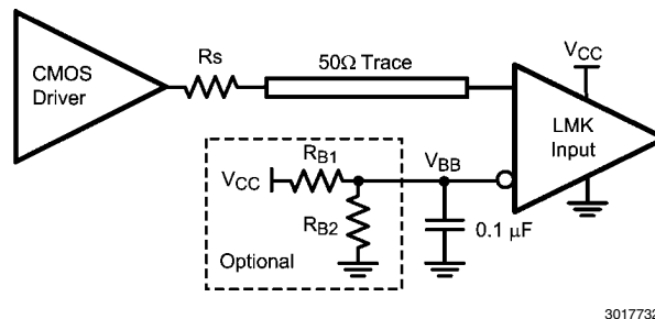
FIGURE 4. Single-Ended LVCMOS Input, DC Coupling with Common Mode Biasing
