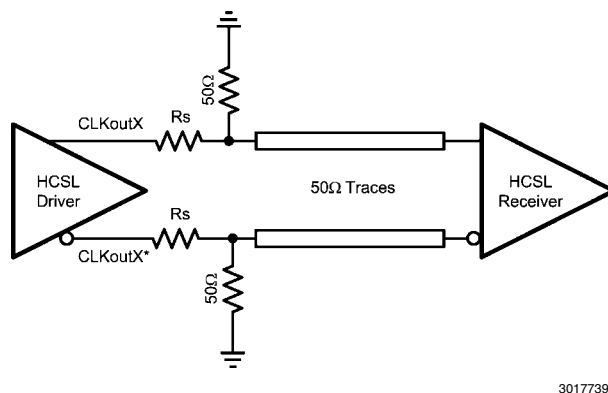
FIGURE 8. HCSL Operation, DC Coupling
