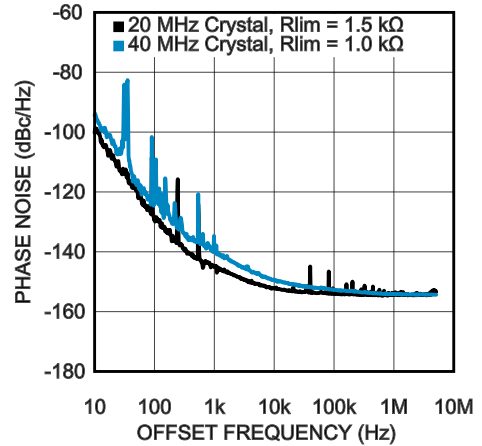
LVDS Phase Noise in Crystal Mode (Note 27, Note 28)
