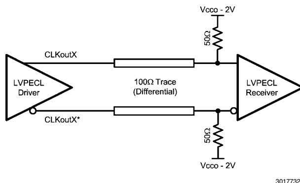
FIGURE 9. Differential LVPECL Operation, DC Coupling
