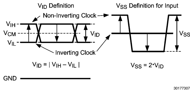
FIGURE 1. Two Different Definitions for Differential Input Signals
