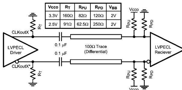
FIGURE 12. Differential LVPECL Operation, AC Coupling, Thevenin Equivalent
